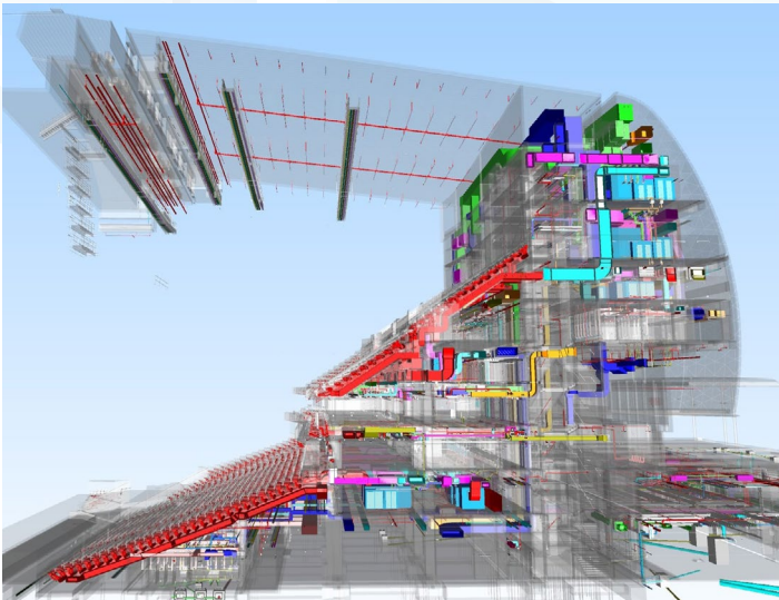
Partial cross-sectional view of the Main Stadium of Kai Tak Sports Park
